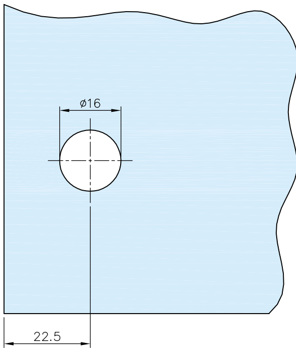
glass cutout
